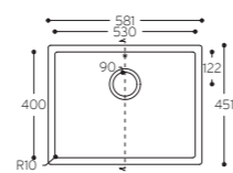
TOP VIEW * overflow
