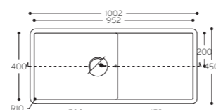
TOP VIEW * overflow
